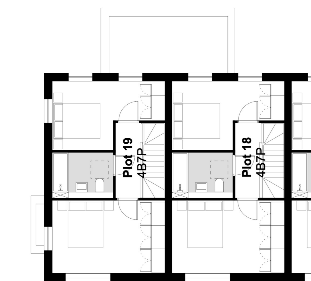
4 Bed House A - Second Floor Plan
