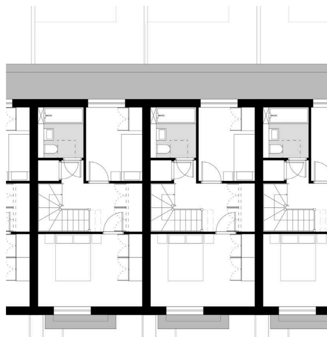
4 Bed House B - First Floor Plan
