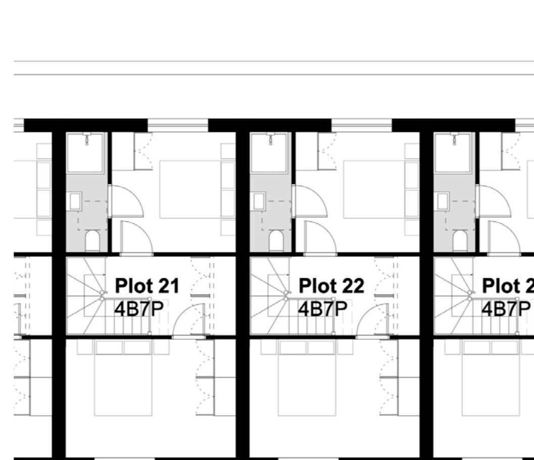
4 Bed House B - Second Floor Plan
